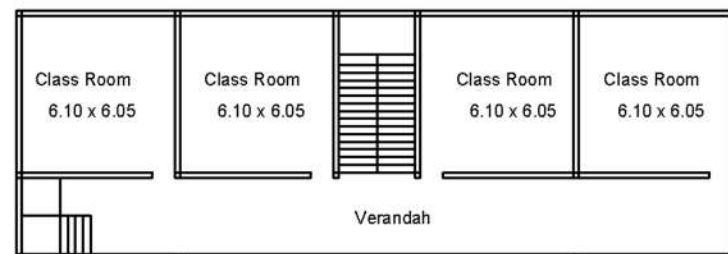
GROUND FLOOR
