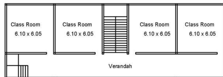
FIRST FLOOR
